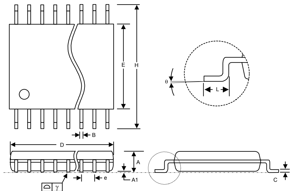
Figure 18. 24-Pin Thin Shrink Small Outline Package (TSSOP)
